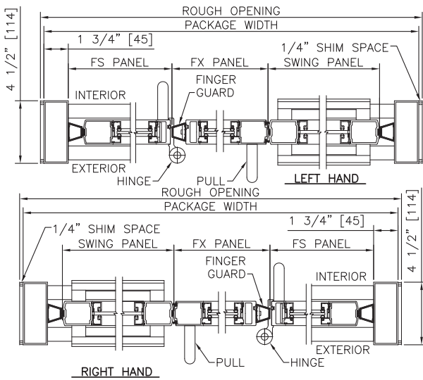
PLAN VIEW SCALE: 3/8" = 1'-0"
