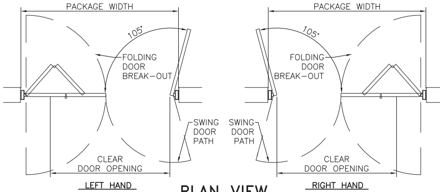
PLAN VIEW SCALE: 3/8" = 1'-0"
