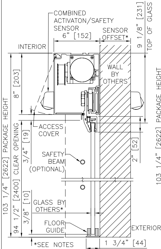
1 VERTICAL SECTION
