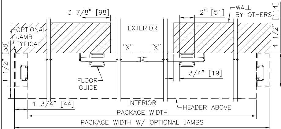
2 HORIZONTAL SECTION
