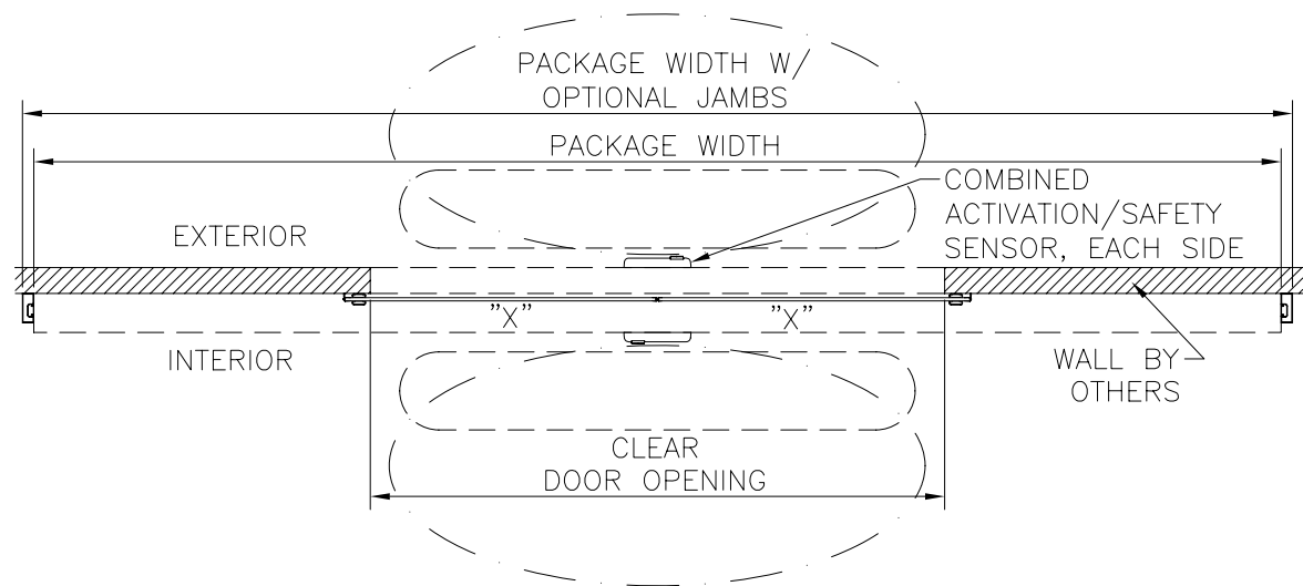
PLAN VIEW SCALE: 3/8" = 1'-0"
