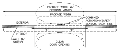
Bi-Part Plan View
