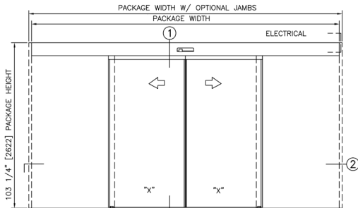
Bi-Part Elevation View
