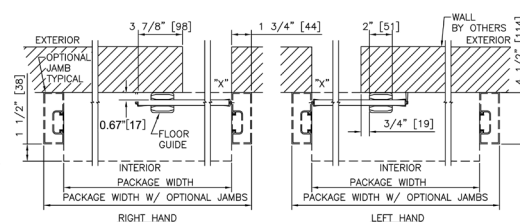
Single Slide Horizontal Section
