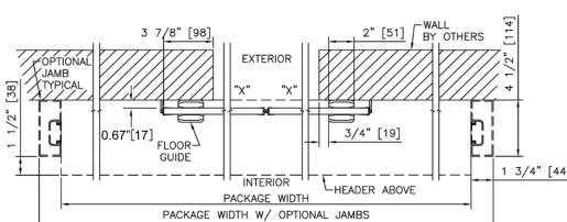
Bi-Part Horizontal Section
