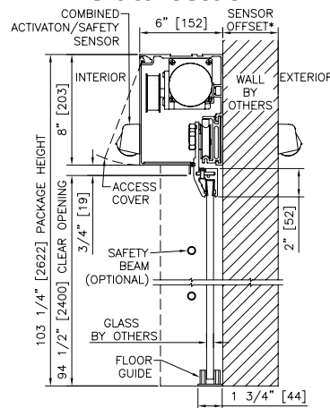
Bi-Part and Single Slide Vertical Section
