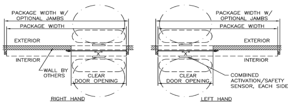
Single Slide Plan View
