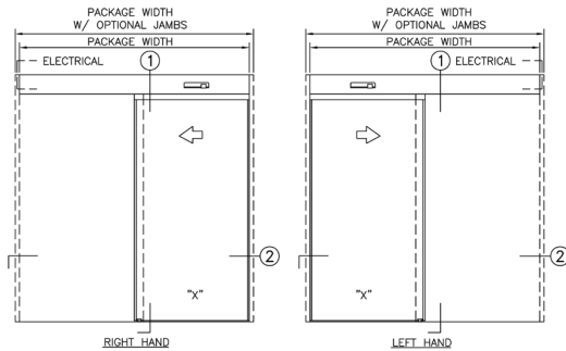
Single Slide Elevation View
