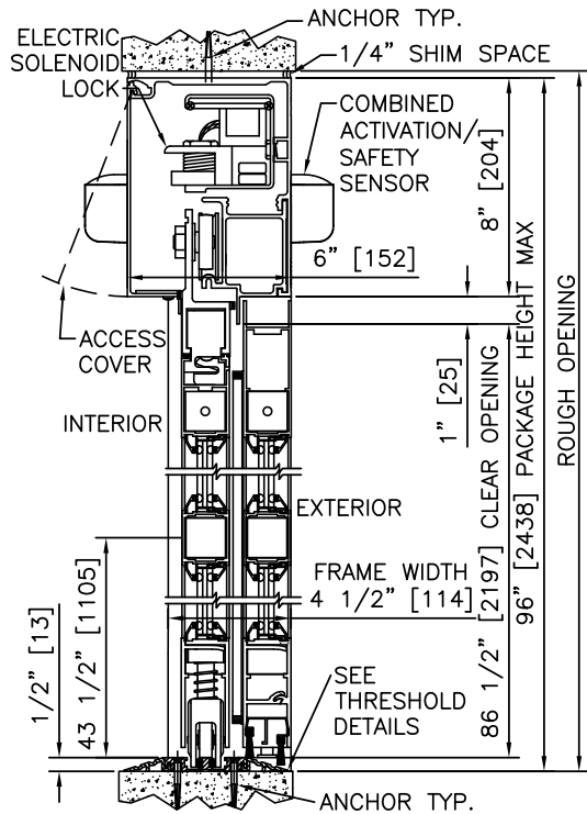
1 VERTICAL SECTION
