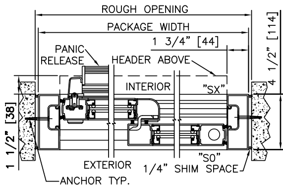
2 HORIZONTAL SECTION
