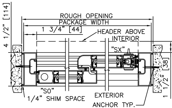
2 HORIZONTAL SECTION
