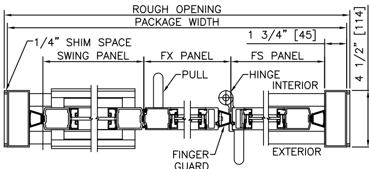
② HORIZONTAL SECTION
