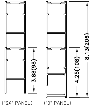
NOMINAL 8"
