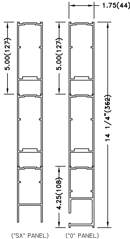
NOMINAL 15"
