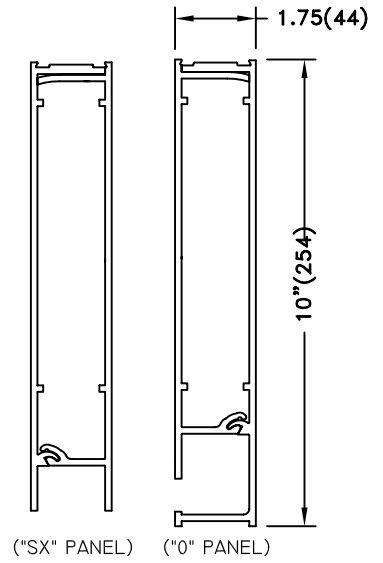
10" SEAMLESS
