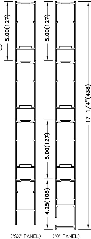
NOMINAL 18"
