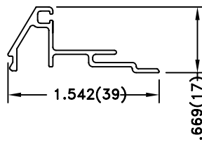
GUTTER-BEVELED EXTRUSION
