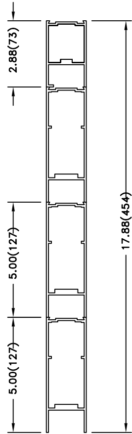
NOMINAL 18"
