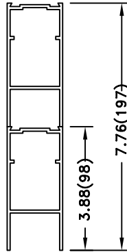
NOMINAL 8"
