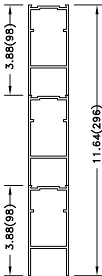
NOMINAL 12"
