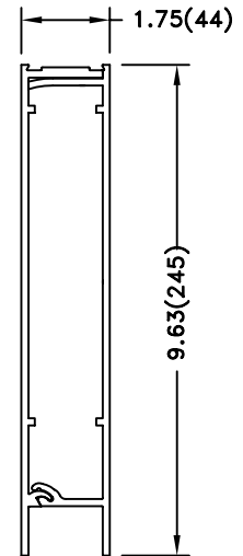
10" SEAMLESS
