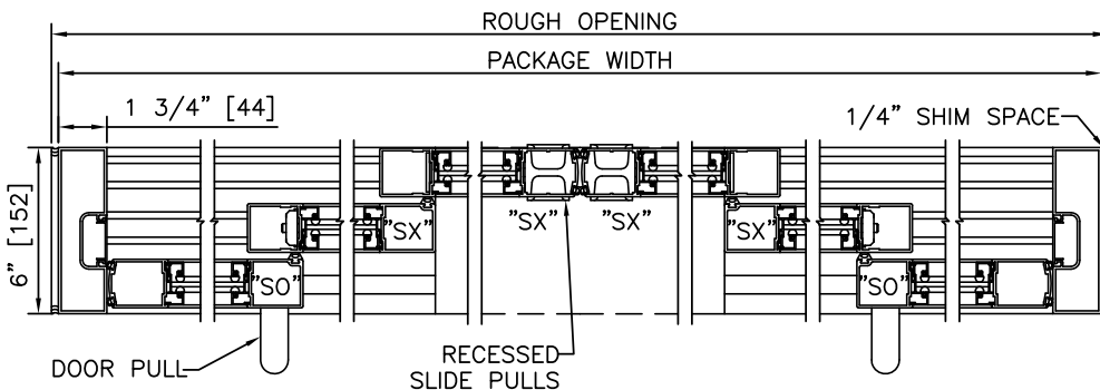
2 HORIZONTAL SECTION
