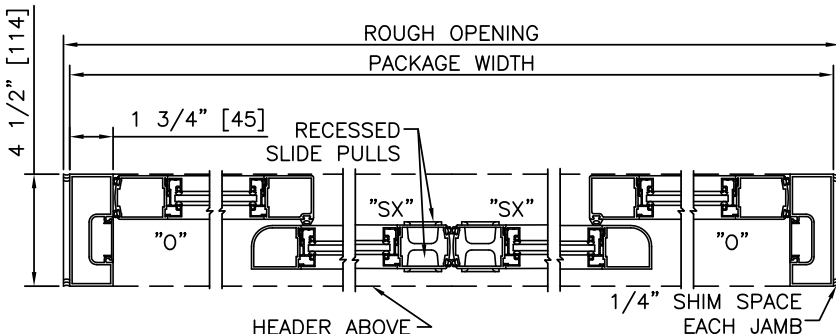
2 HORIZONTAL SECTION
