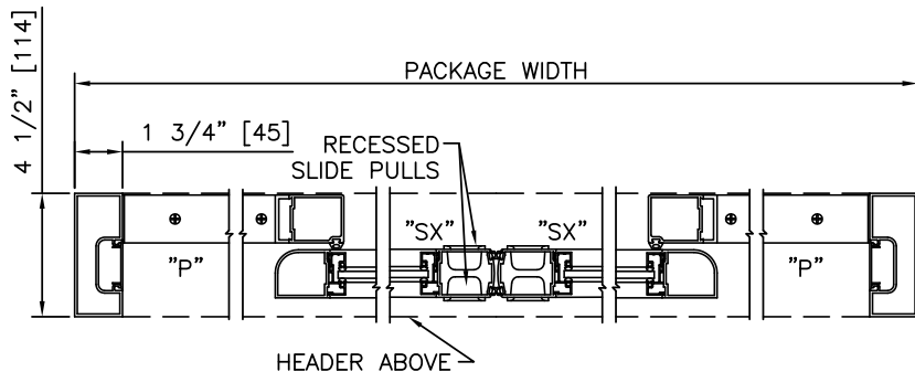
2 HORIZONTAL SECTION
