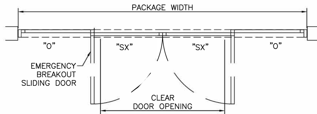
PLAN VIEW SCALE: 3/8" = 1'-0"
